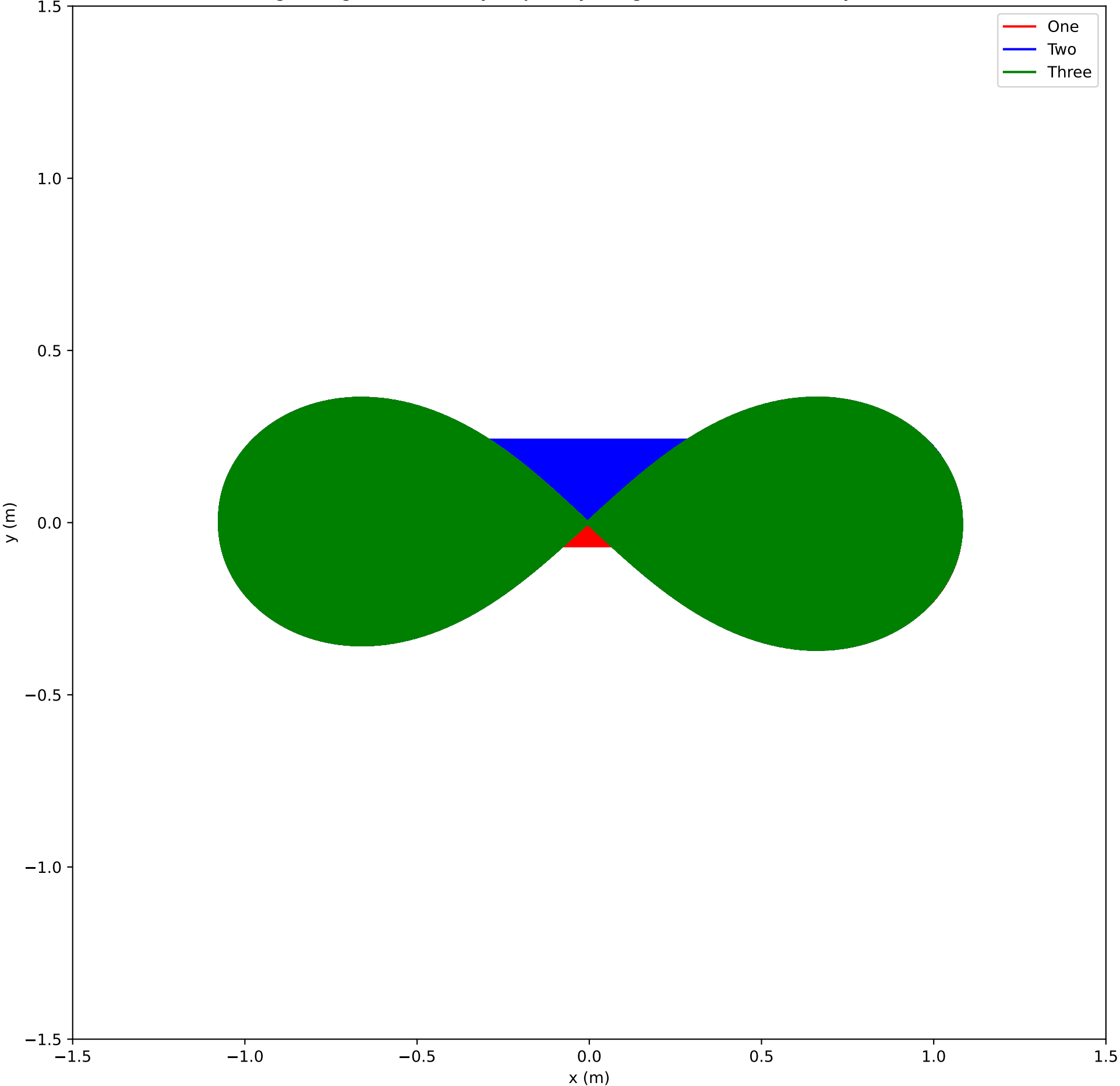
Stable (Figure-Eight) Three-Body Trajectory Integrated with the Velocity Verlet Method
